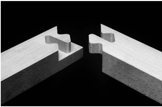
Figure 6: Digital wood joint : a corner connection, designed by C-Lab, 1997.
