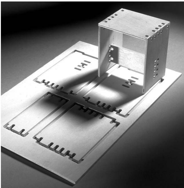
Figure 7: C-Stool , a CNC-compatible redesign of a three-board stool, designed by Jochen Gros, 1994.
