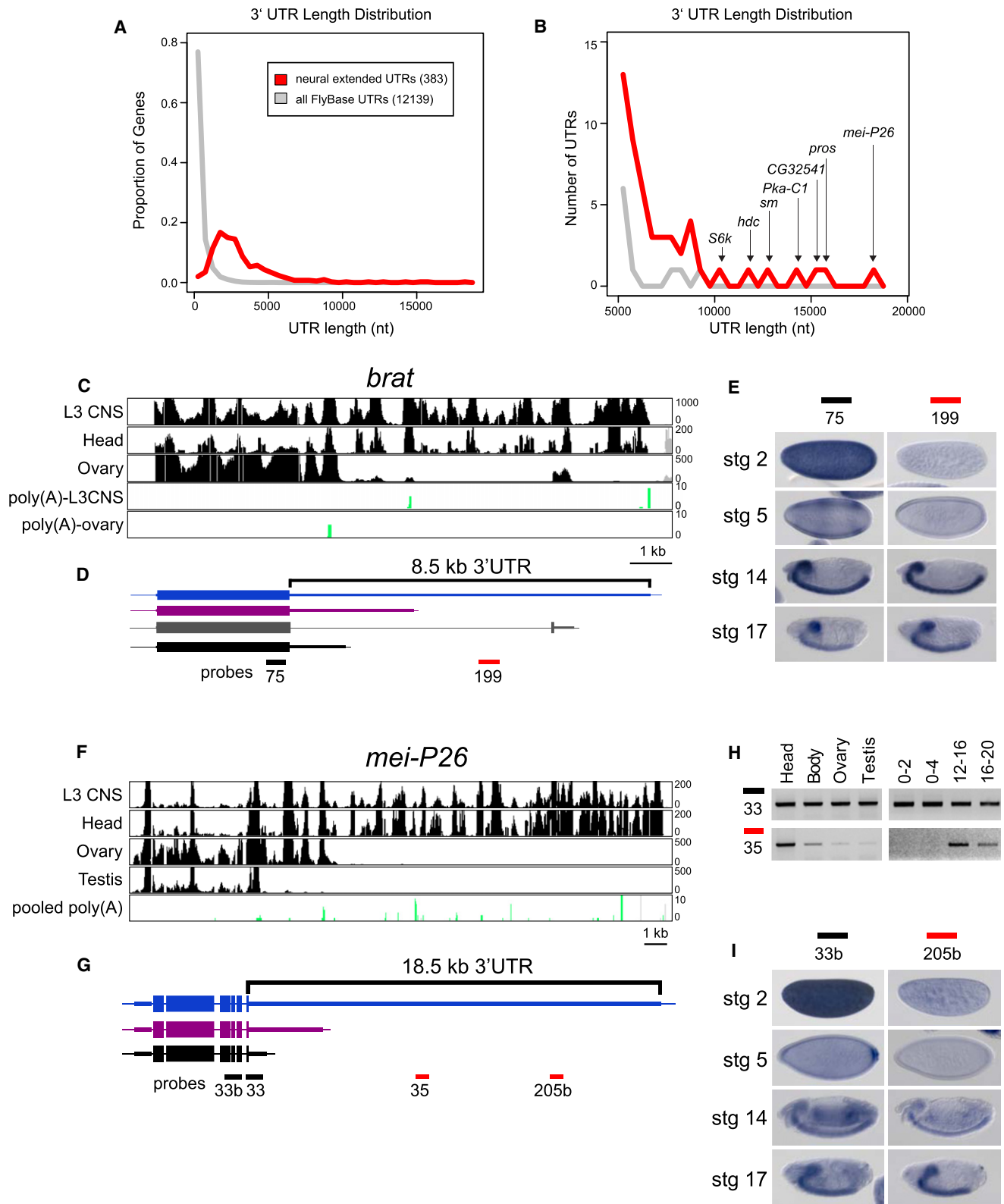
Figure 3. Unusually Long 3' UTR Extensions in Neural Genes
