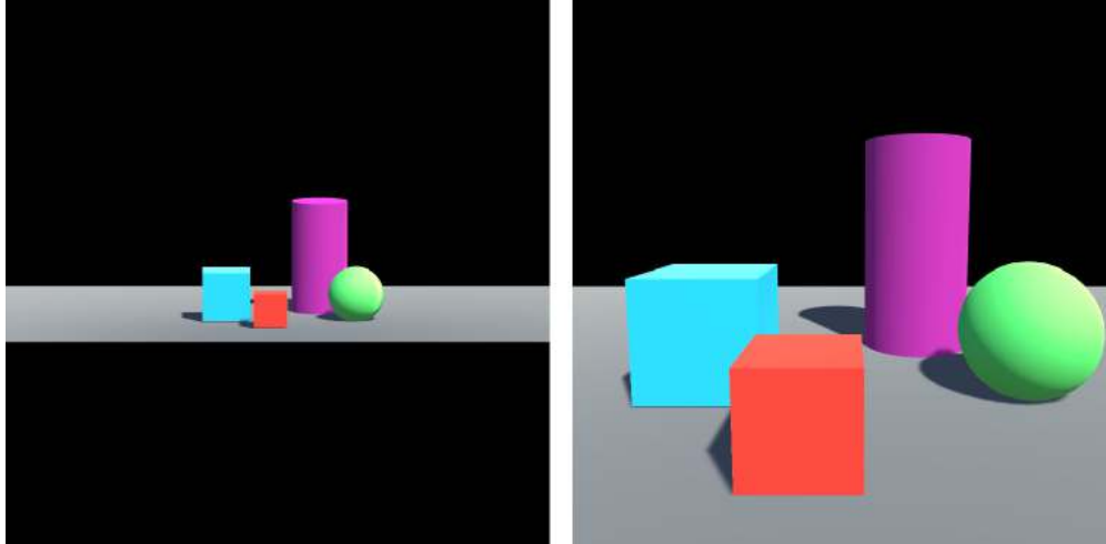
Figure 3.5: The same scene rendered with an orthographic projection (left) and a perspective projection (right).
