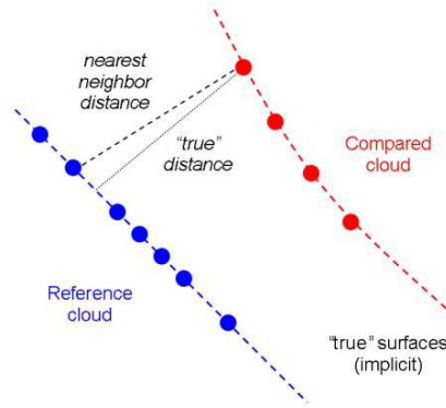
Figure 4.16: An example distance calculation from CloudCompare [230].
