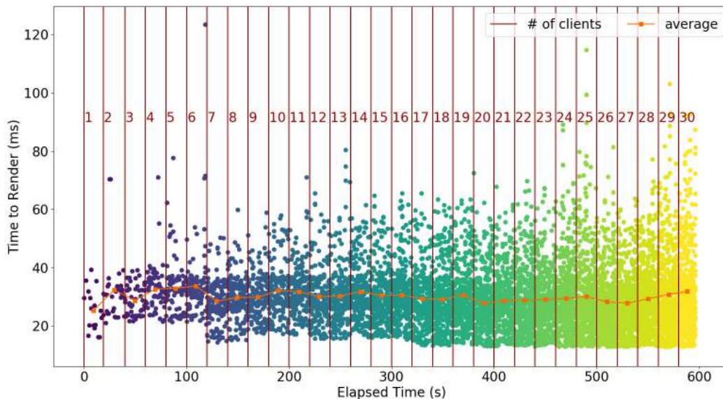
Figure 4.20: A plot of response times as the number of clients making requests is increased incrementally, up to 30 clients.
