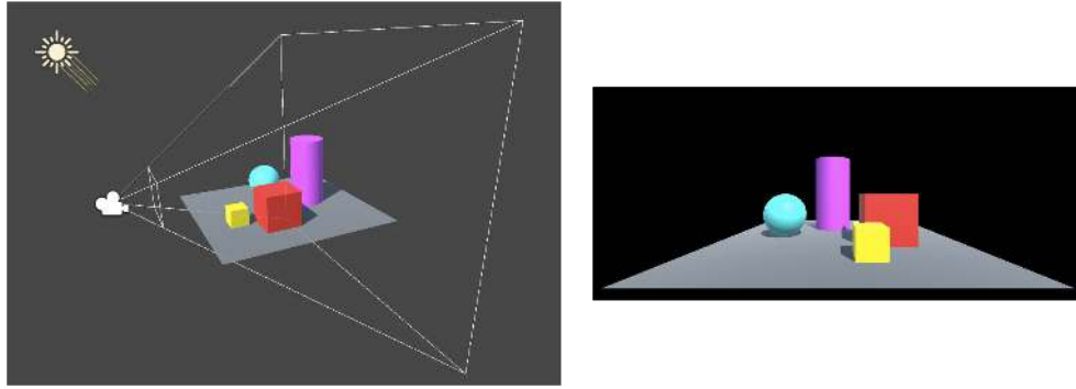
Figure 3.4: An example scene with camera, light, and 3D objects (left) and rendered image (right) using the synthetic camera model.
