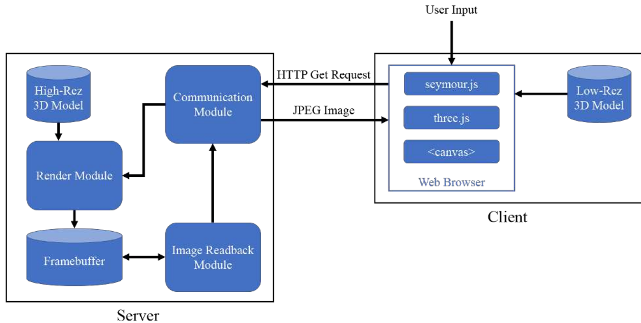
Figure 4.4: The system architecture of Seymour.
