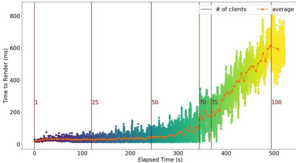
Figure 4.22: A plot of response times as the number of clients making requests is increased incrementally, up to 100 clients.
