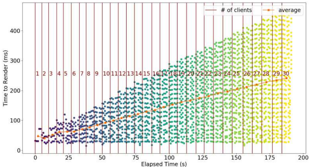
Figure 4.21: A plot of response times as the number of clients making concurrent requests is increased incrementally.
