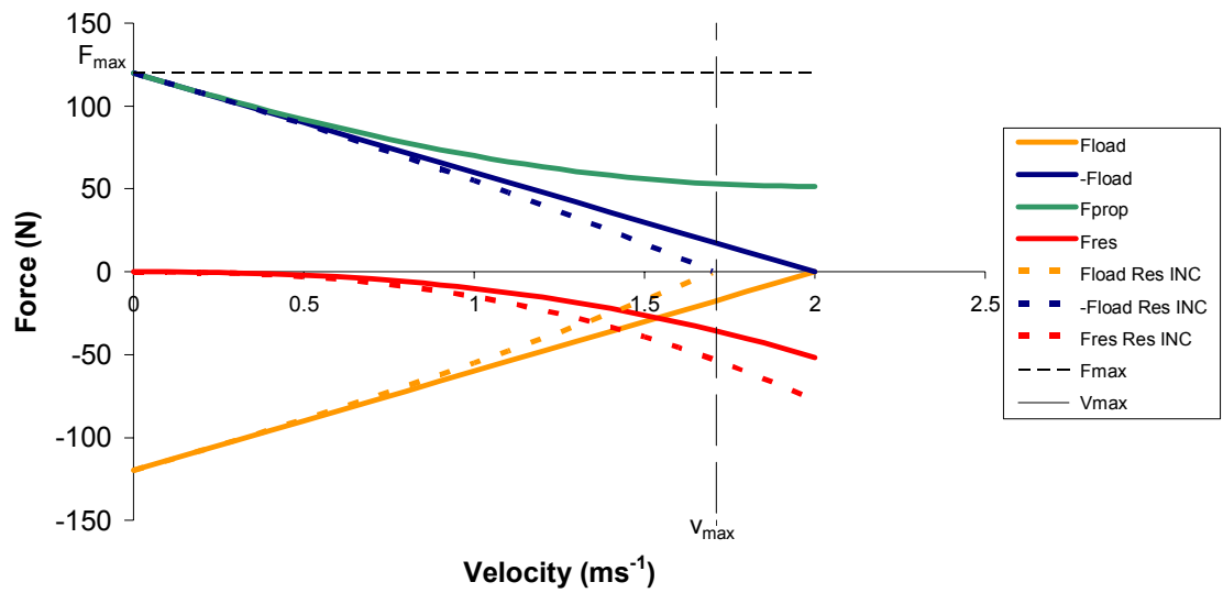
FIGURE 5 - Theoretical effect of an increase of F_{res} on F_{max} , v_{max} , and the relationship of F_{load} to velocity
