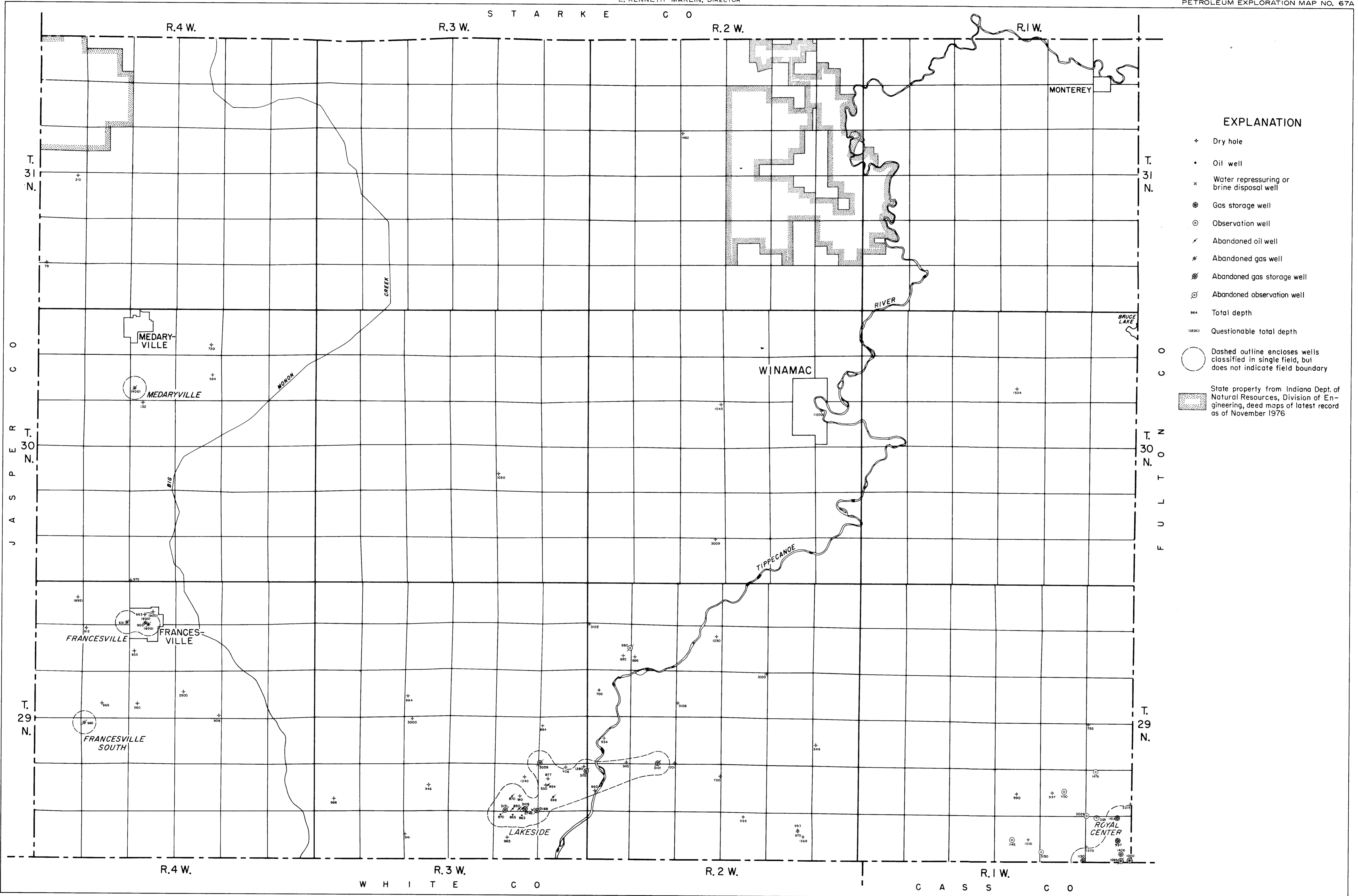
WELL LOCATION MAP OF PULASKI COUNTY, INDIANA, SHOWING TOTAL DEPTH OF WELLS
