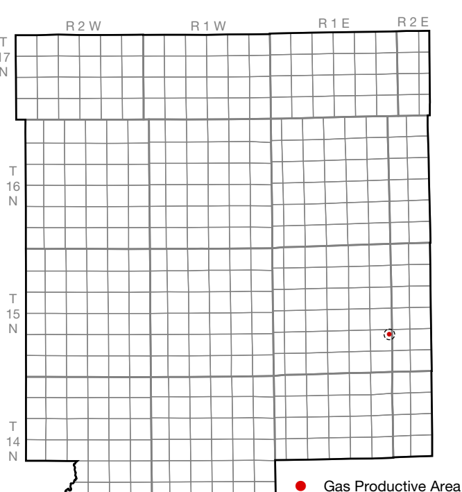
Index map of Hendricks County showing petroleum field boundaries and gas productive areas
