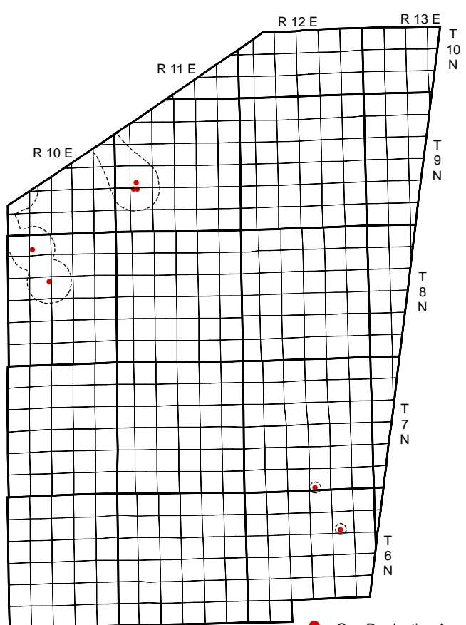
Index map of Ripley County showing petroleum field boundaries and gas productive areas
