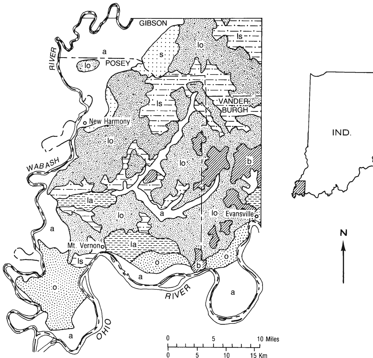
Figure 8. Quaternary geologic map of the field-trip area, generalized from Gray (in preparation). a, alluvium; s, dune sand; lo, loess; la, lacustrine deposits; ls, lowland silt complex; o, outwash sand; b, bedrock. All deposits mapped are Late Wisconsinan in age except alluvium, which is Holocene, and bedrock, which is Pennsylvanian.
