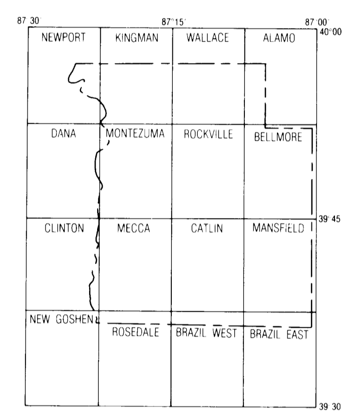
Index map of Parke County showing U.S. Geological Survey 7 1/2' topographic quadrangle map names
