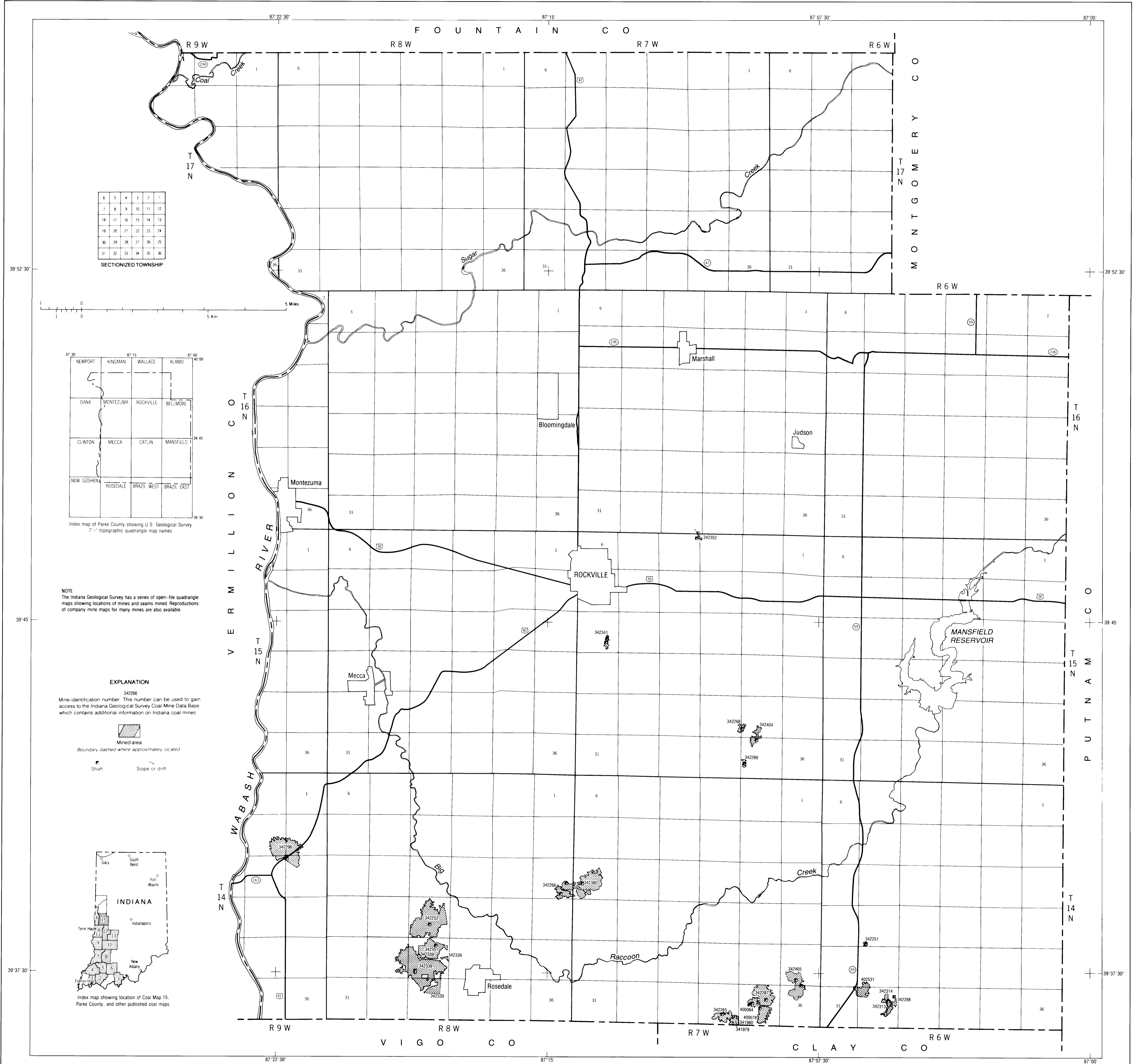
MAP OF PARKE COUNTY, INDIANA, SHOWING LOCATIONS OF UNDERGROUND COAL MINES
