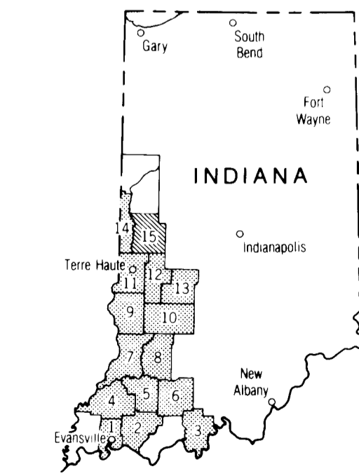
Index map showing location of Coal Map 15, Parke County, and other published coal maps.
