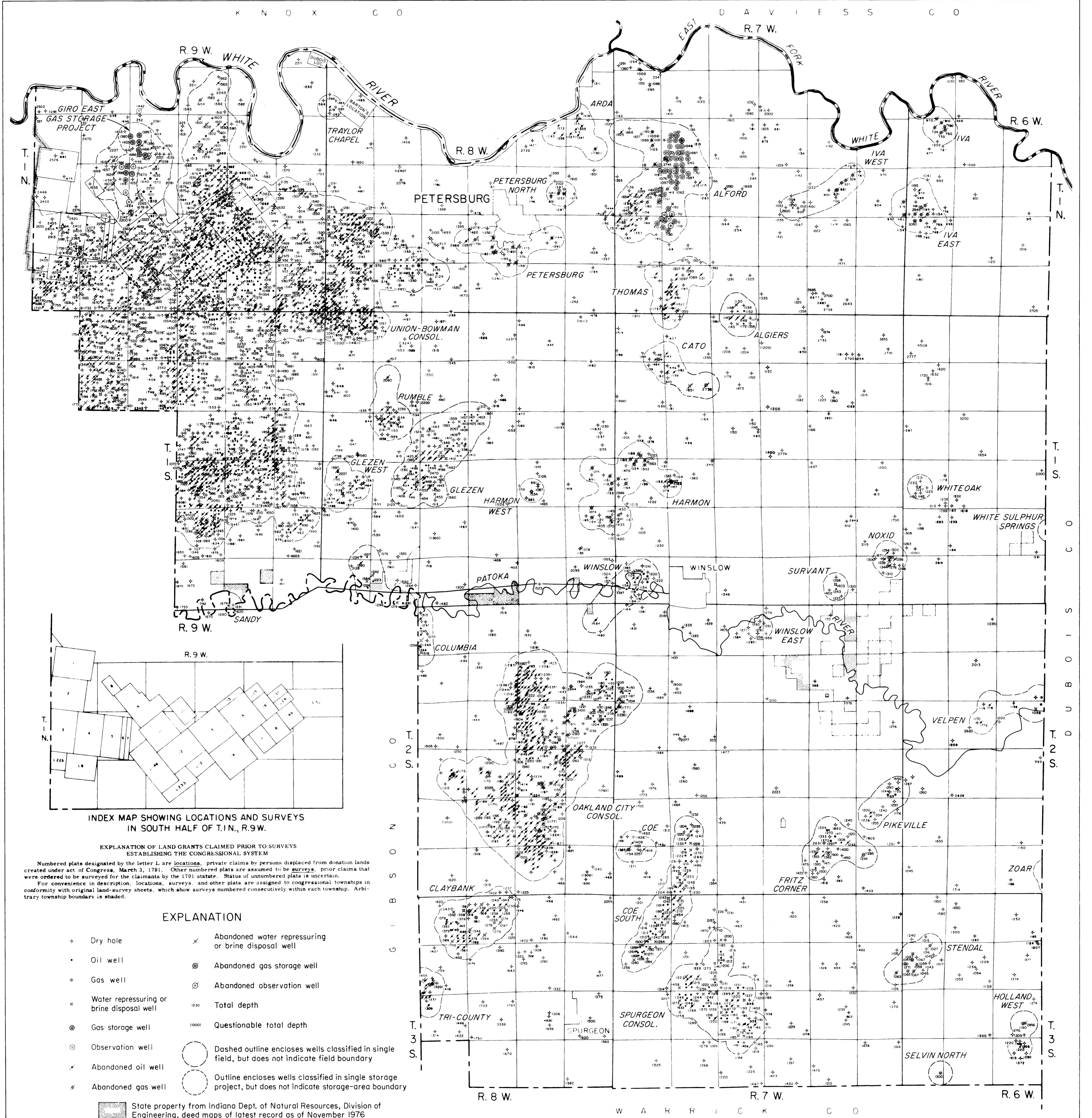
WELL LOCATION MAP OF PIKE COUNTY, INDIANA, SHOWING TOTAL DEPTH OF WELLS
