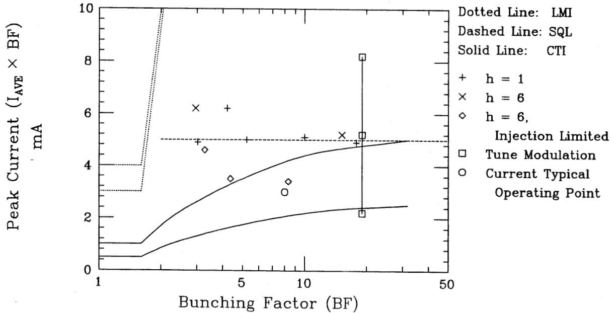
Figure 1. Instability limits in the IUCF Cooler for electron-cooled 45-MeV proton beams.
