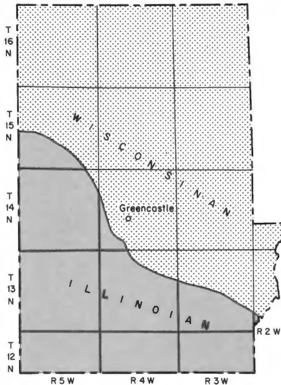
Figure 2. Map of Putnam County showing general distribution of Wisconsin and Illinoian glacial deposits. Modified from Malott, 1922.
