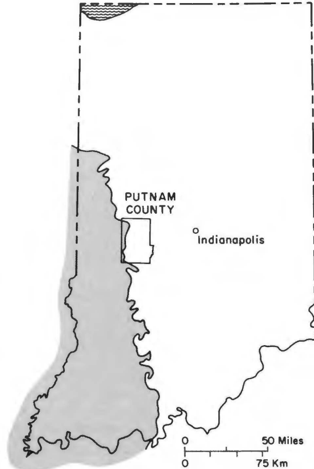
Figure 6. Map of Indiana showing the eastern part of the Illinois Basin.
